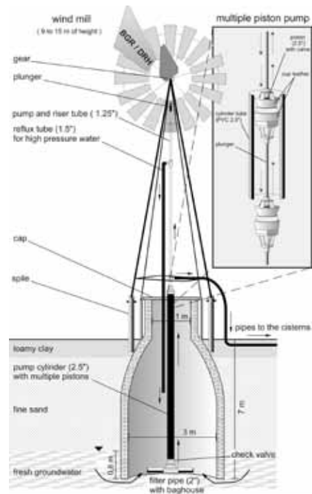
Figure 31. Schematic overview of windmill.
